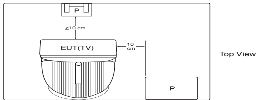
Figure 6—Test arrangement for radiated emissions (table-top equipment)
