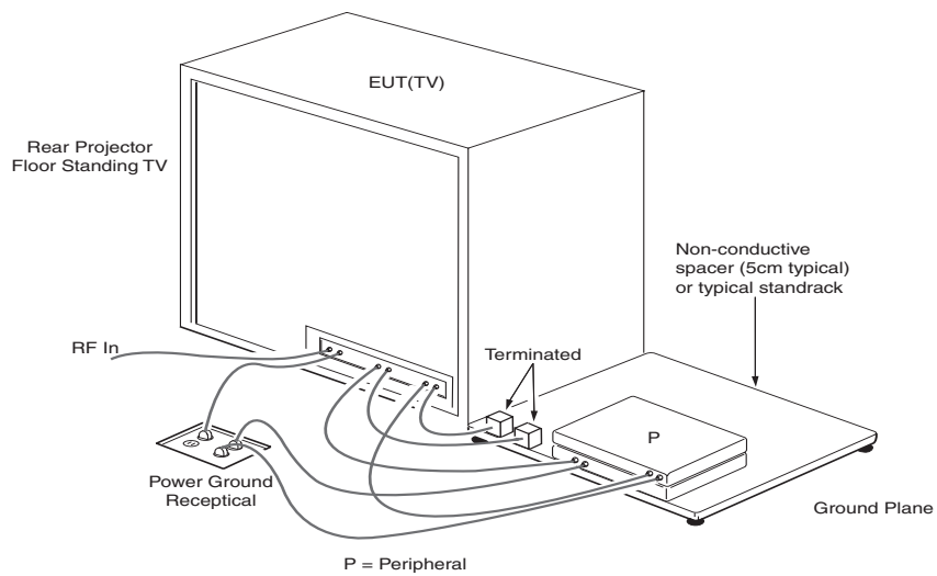
Figure 7—Test arrangement for radiated emissions (floor-standing equipment)
