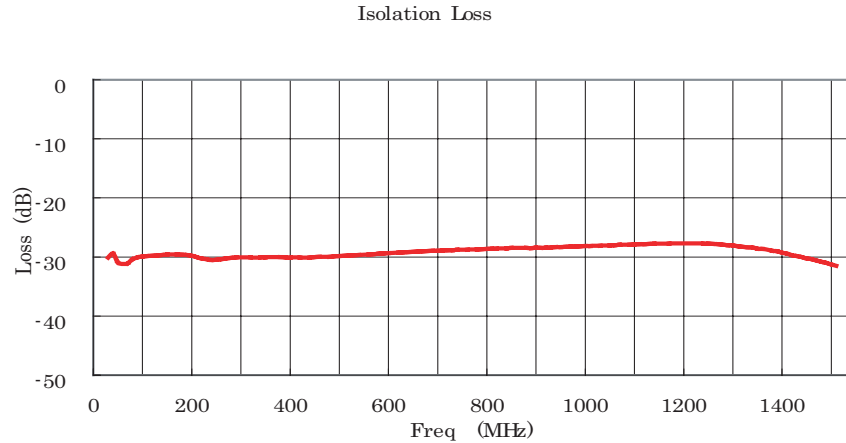
Figure 3—Typical characteristic of insertion loss of isolation transformer for 46 MHz to 1.5 GHz
