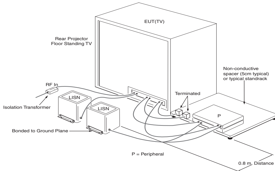
Figure 5—Test arrangement for conducted emissions (floor-standing equipment)
