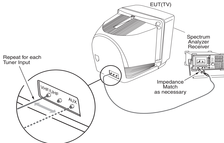
Figure 8—Test arrangement for antenna radiation
