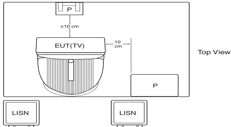
Figure 4—Test arrangement for conducted emissions (table-top equipment)
