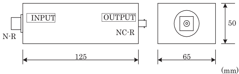
Figure 2—Typical size of isolation transformer for 46 MHz to 1.5 GHz
